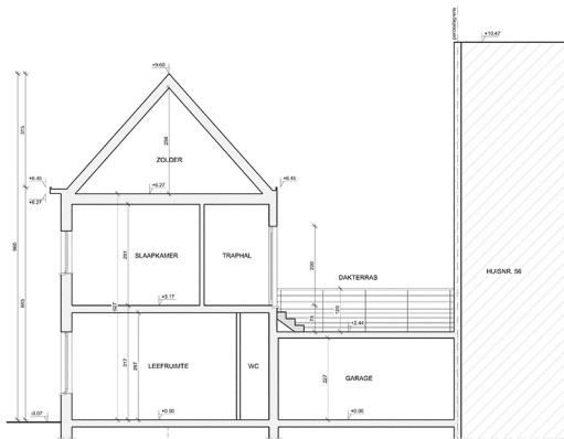
DOORSNED E B-B
