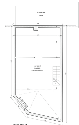
ZOLDER
